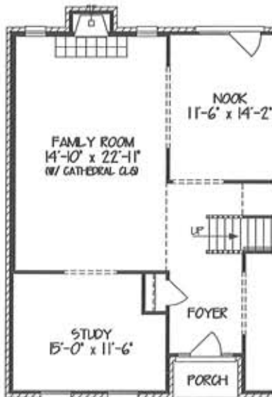
OPTIONAL FIRST FLOOR PLAN 'B' (INCLUDES LIVING ROOM VS. FULL FRONT PORCH) ADDS 126 SF
