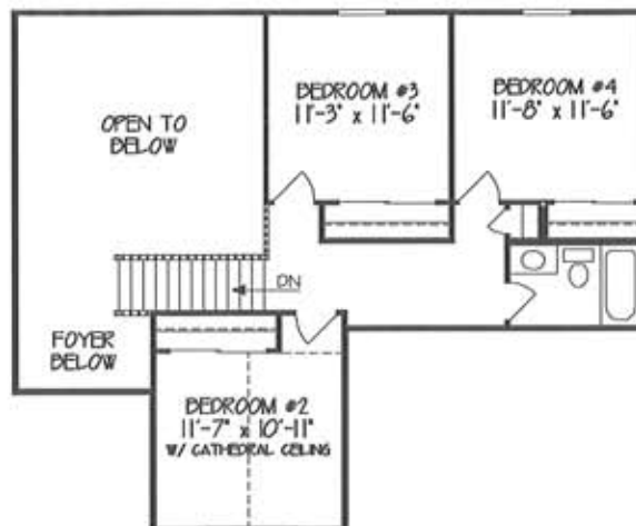
SECOND FLOOR PLAN 678 SF
