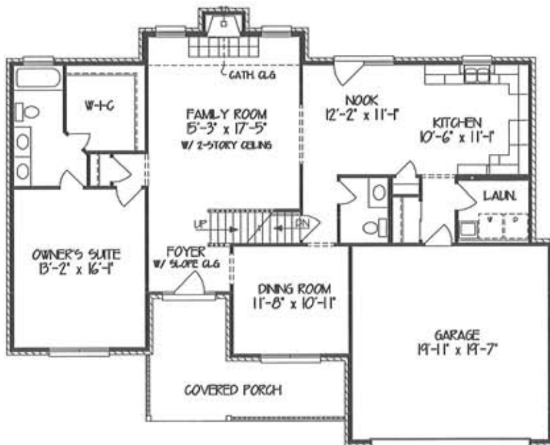
FIRST FLOOR PLAN 1396 SF
