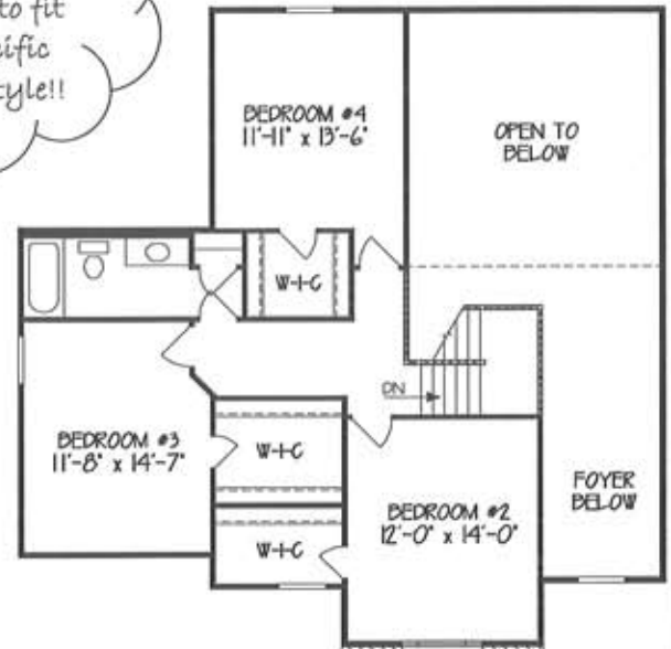
SECOND FLOOR PLAN 920 SF
