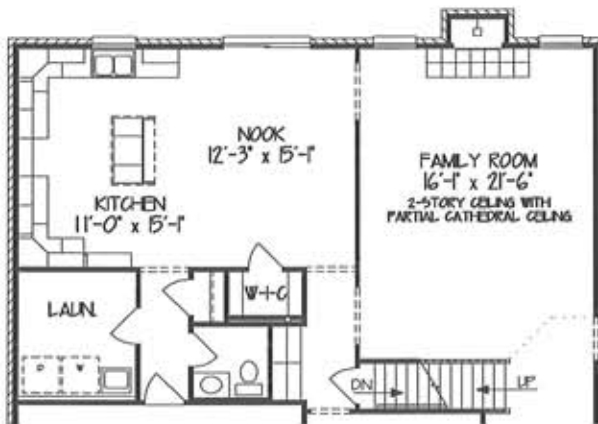
OPTIONAL STAIR LAYOUT W/ BUTLER'S PANTRY VS. DESK UNIT
