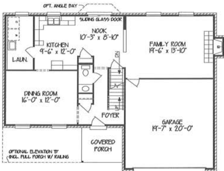
FIRST FLOOR PLAN 1003 SF
