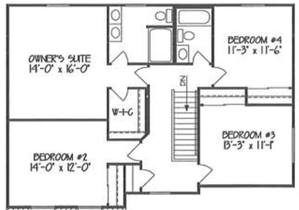
OPTIONAL SECOND FLOOR PLAN 'C' (INCL. DOUBLE GABLE FRONT)
