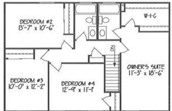
SECOND FLOOR PLAN 1014 SF
