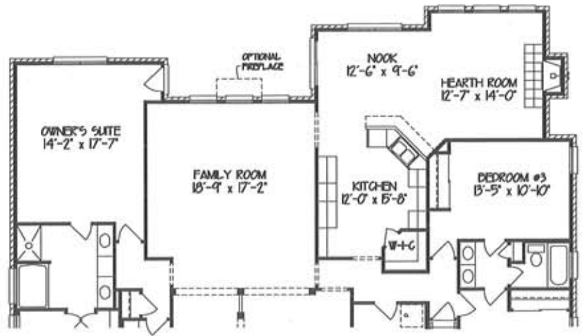
OPTIONAL FIRST FLOOR PLAN (INCLUDES HEARTH ROOM & ALTERNATE KITCHEN LAYOUT) ADDS 129 SF
