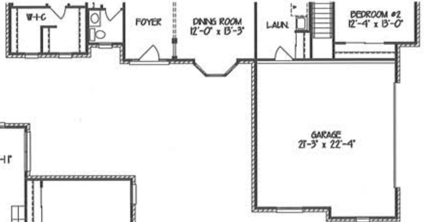
OPT. FIRST FLOOR PLAN 'C' (INCL. 10' CEILINGS AT FOYER & DINING ROOM W/ BRICK GABLE FRONT & ANGLE BAY) ADDS 12 SF
